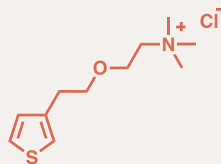
Thiophene methanol chlorine ethyl-trimethylammonium
