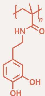
Poly((3,4-dihydroxyphenylethyl)-2-propenamamide)
