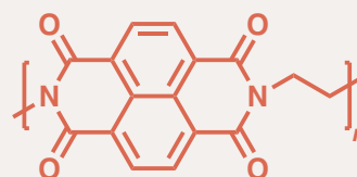
Poly(naphthalene-4-formylethylenediamine)
