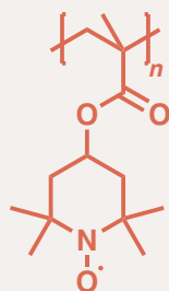
Poly((2,2,6,6-Tetramethylpiperidin-1-oxyl methacrylate)
