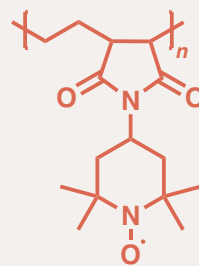
Poly(ethylene-alt-maleic anhydride)-(2,2,6,6-Tetramethylpiperidin-1-oxyl)
