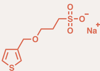
Thiophene methanol sodium propane sulfonate
